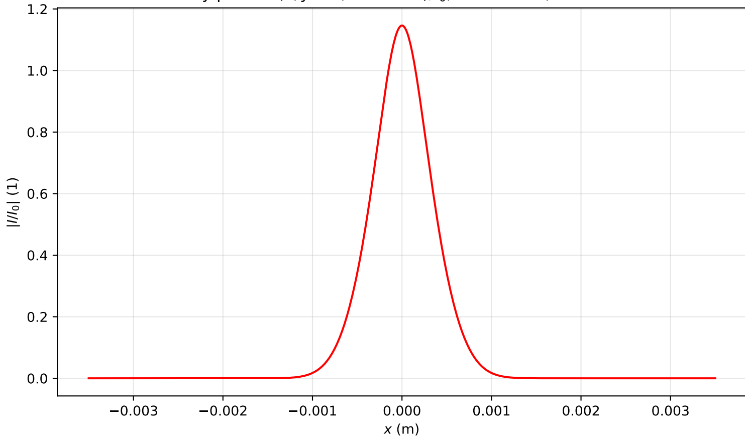
Intensity profile I(x, y = 0, z = 0.239)/I_0 , P_{in}=2.5P_{cr} , artificial time
